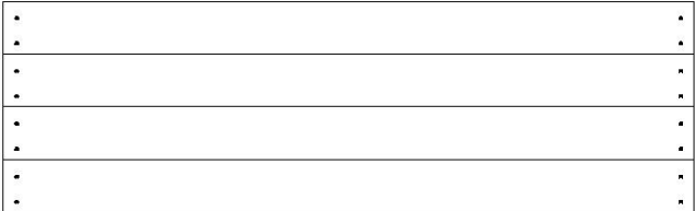
RP1 | PANEL SUPERIOR DEL TECHO - W2A03276 (x2) 1 5/8"x20 5/8"x59" (42x511x1676)
